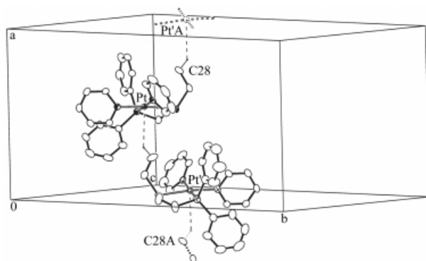
Figure 2. View of crystallographic asymmetric unit showing the intermolecular H bonds between the two independent complexes and the adjacent units translated along the crystallographic a axes ( x \pm 1, y, z ); shaded unit is the complex reported in Figure 1; thermal ellipsoids at the 10% probability level while the hydrogen size is arbitrary
