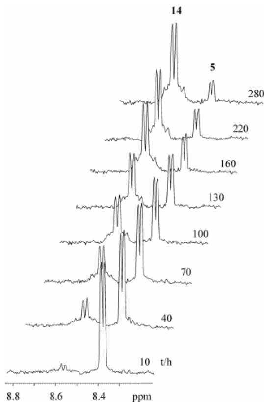
Figure 3. 1 H NMR spectral changes associated with ring closure on cis -[PtPh 2 (CO)(η 1 -ppy)] (5) in CDCl 3 at 298 K; the signals monitored are those of the H 6 -py proton at δ = 8.39 for the ring-open and at δ = 8.55 for the chelate [PtPh 2 (ppy)] (14) complex, respectively
